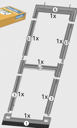
Bi-Lite System - Tile Roof Flashing
