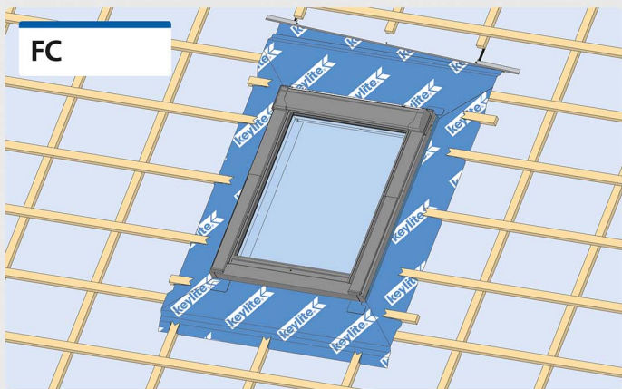
Felt Collar
