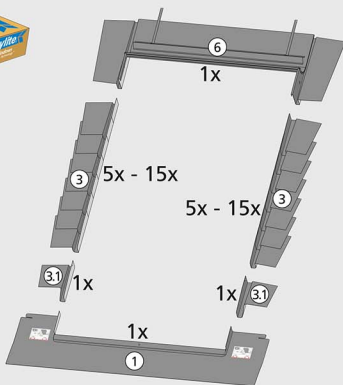
Plain Tile Roof Flashing
